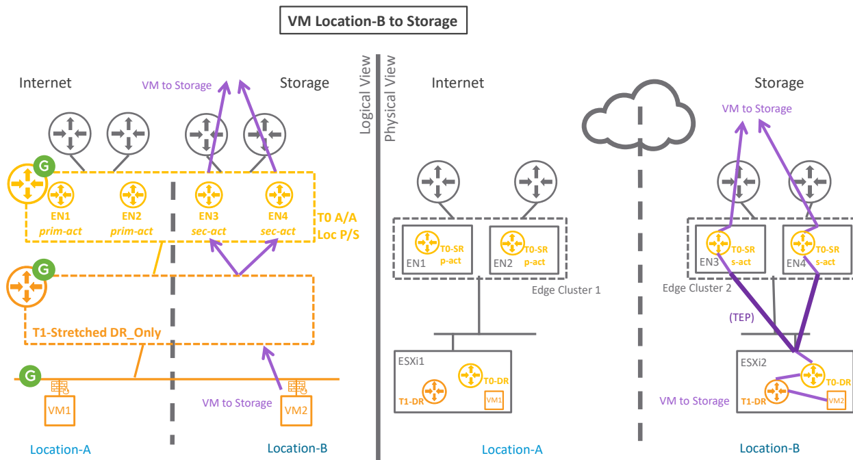
Figure 4-44: NSX-T Federation T0 A/A LocP_S packet walk4
