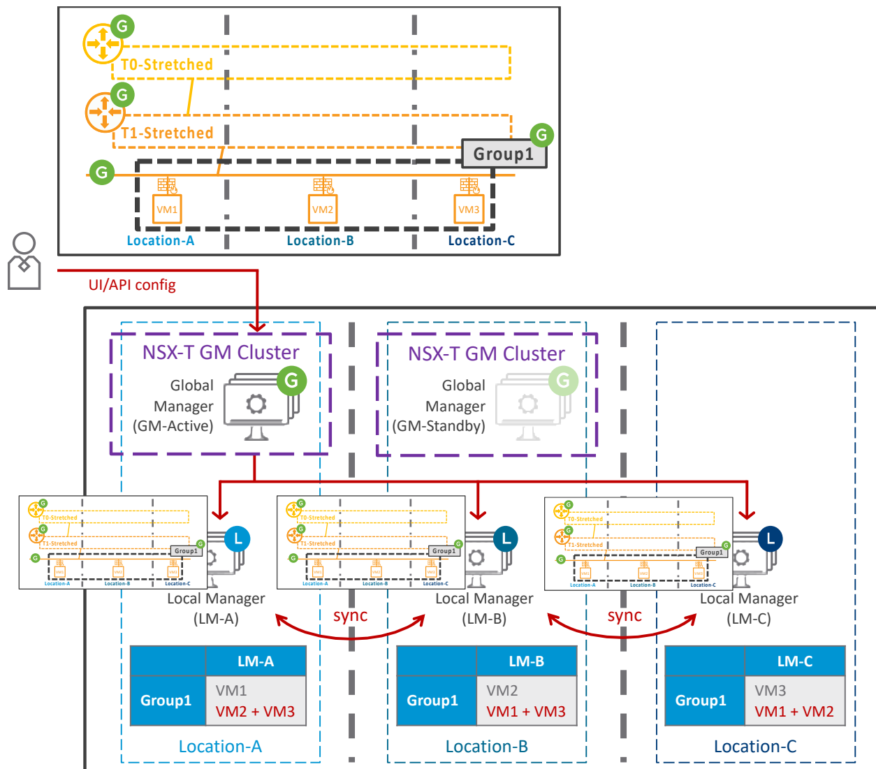
Figure 4-7: LM to LM communication Flow – stretched NSX Group
