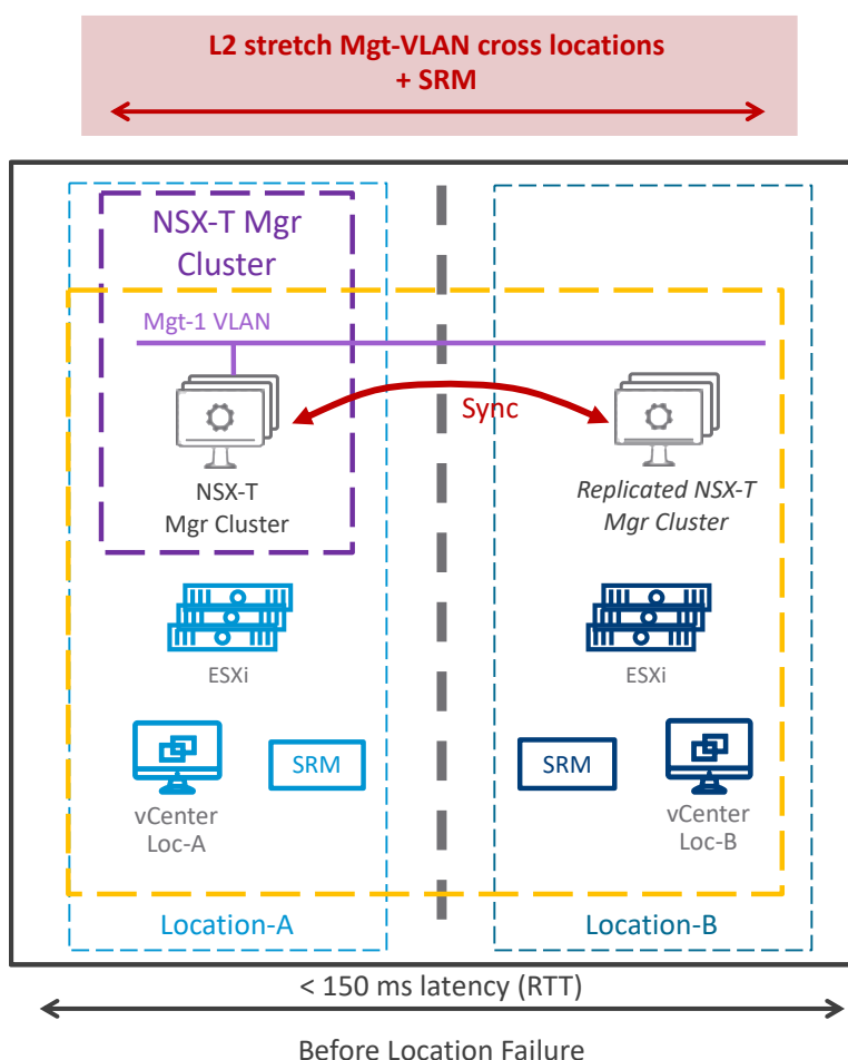
Figure 3-28: Management Plane Deployment Mode2 Option1 with SRM – Before location failure
