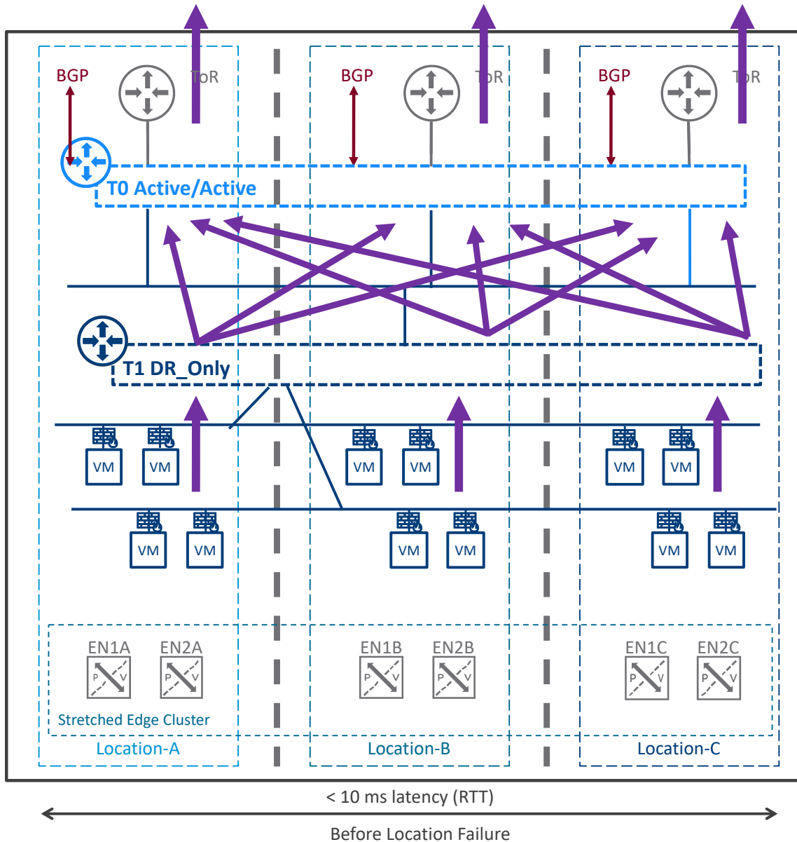
Figure 3-38: Data Plane Deployment Mode3 with Tier1 DR_Only – Before location failure
