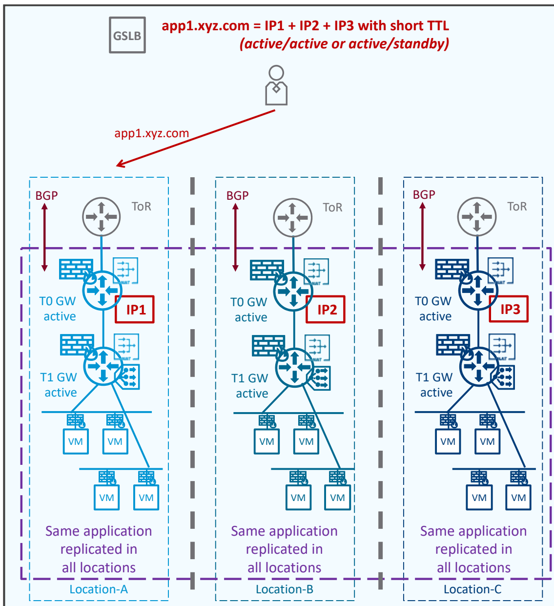
Figure 3-47: GSLB option - Before location failure
