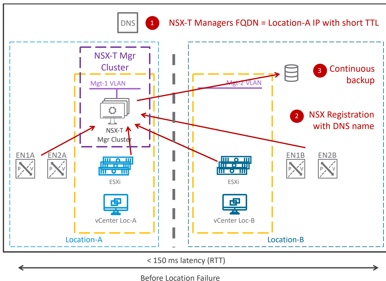
Figure 3-30: Management Plane Deployment Mode2 Option2 – Before location failure
