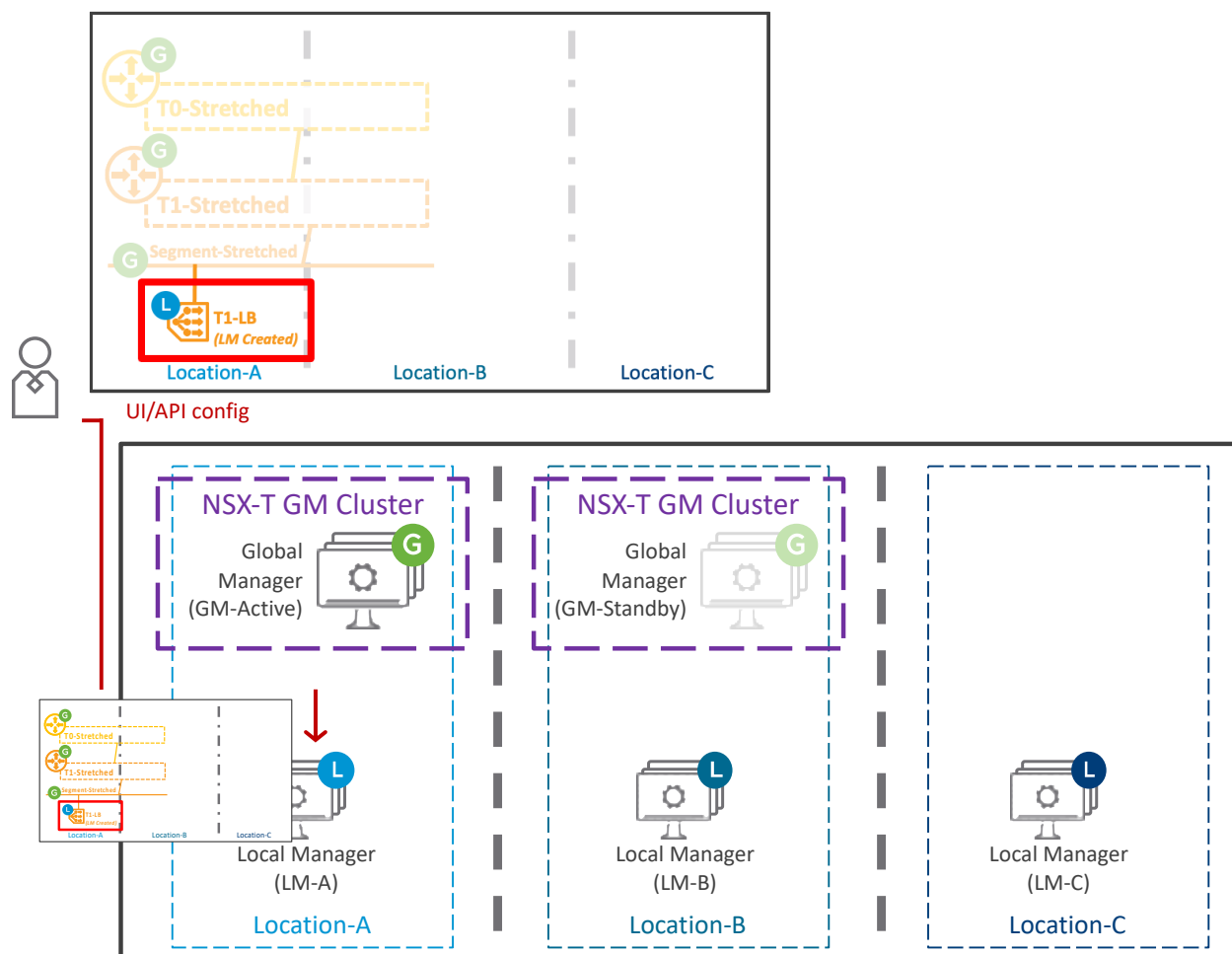
Figure 4-6: Direct LM configuration
