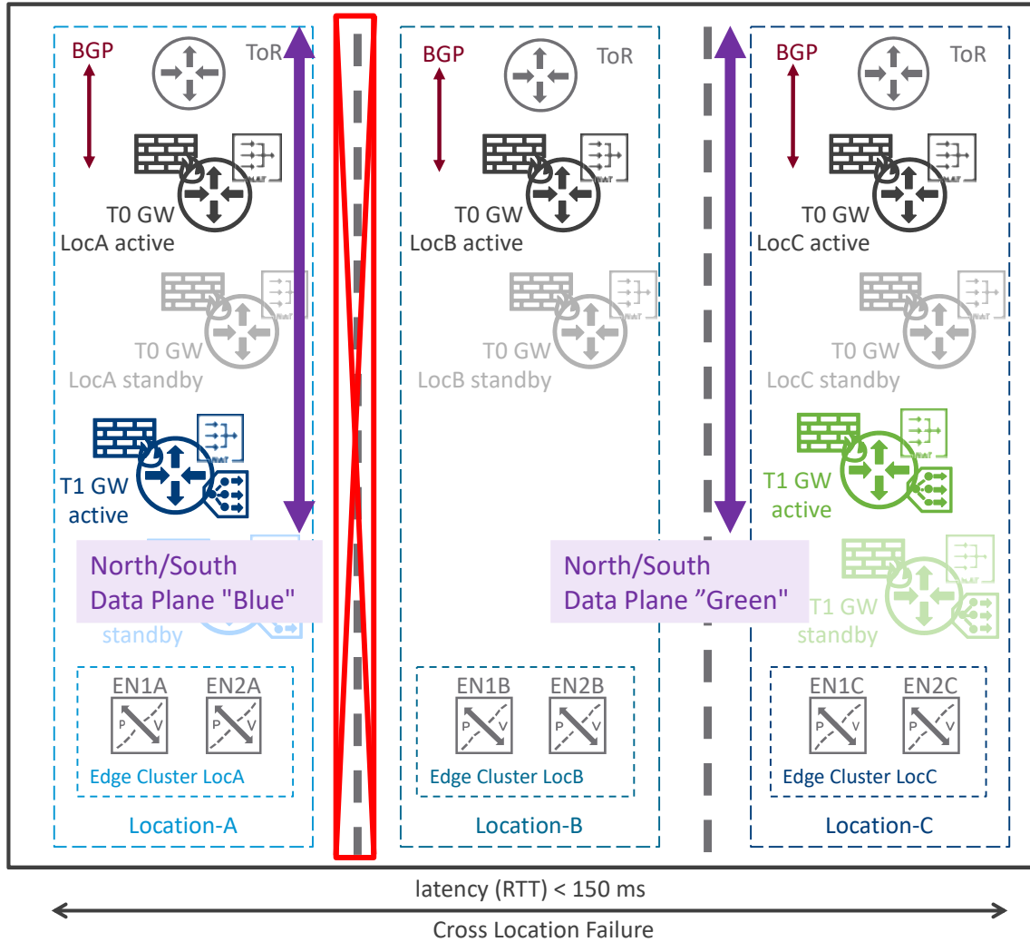
Figure 3-37: Data Plane Deployment Mode2 – After cross-location failure
