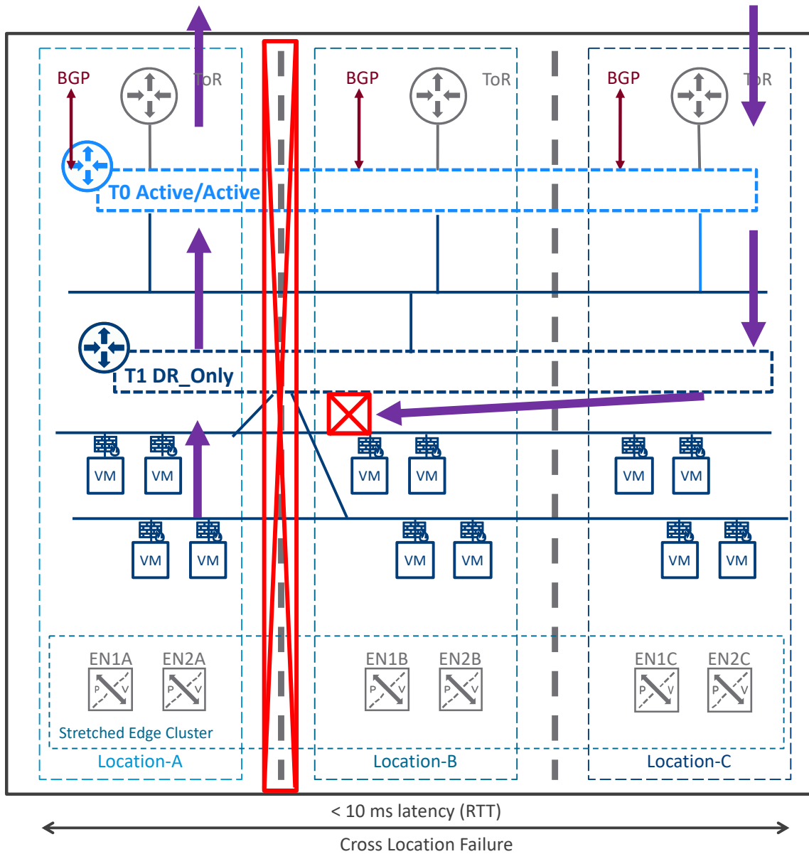
Figure 3-42: Data Plane Deployment Mode3 with Tier1 DR_Only – After cross-location failure
