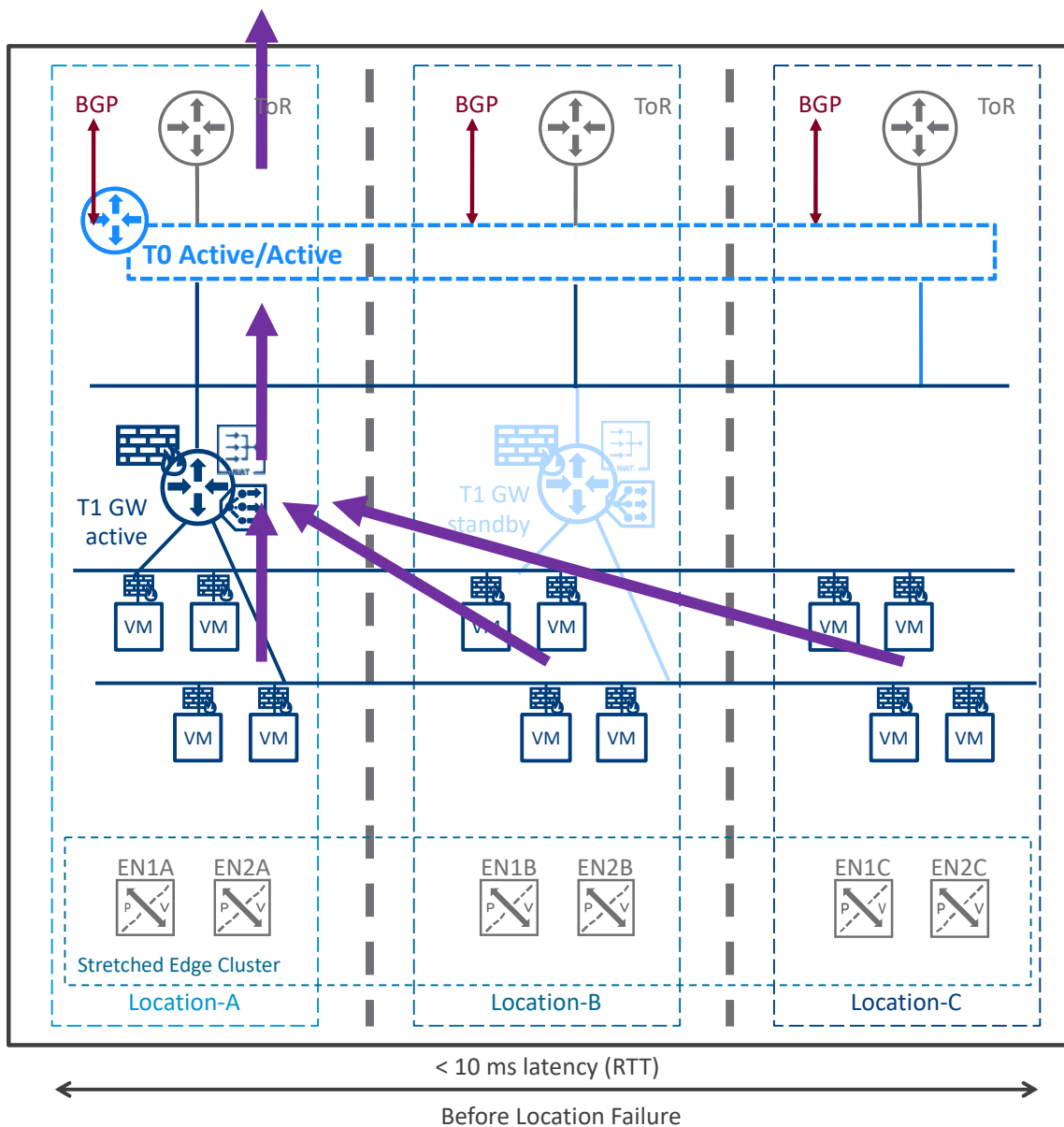
Figure 3-39: Data Plane Deployment Mode3 with Tier1 with Services – Before location failure
