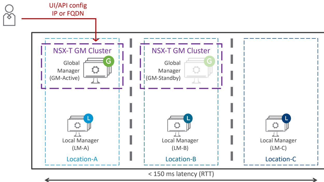
Figure 4-78: NSX-T Multisite Manager Cluster– Use-case two Locations only and/or Data Centers far apart (> 10 ms latency)
