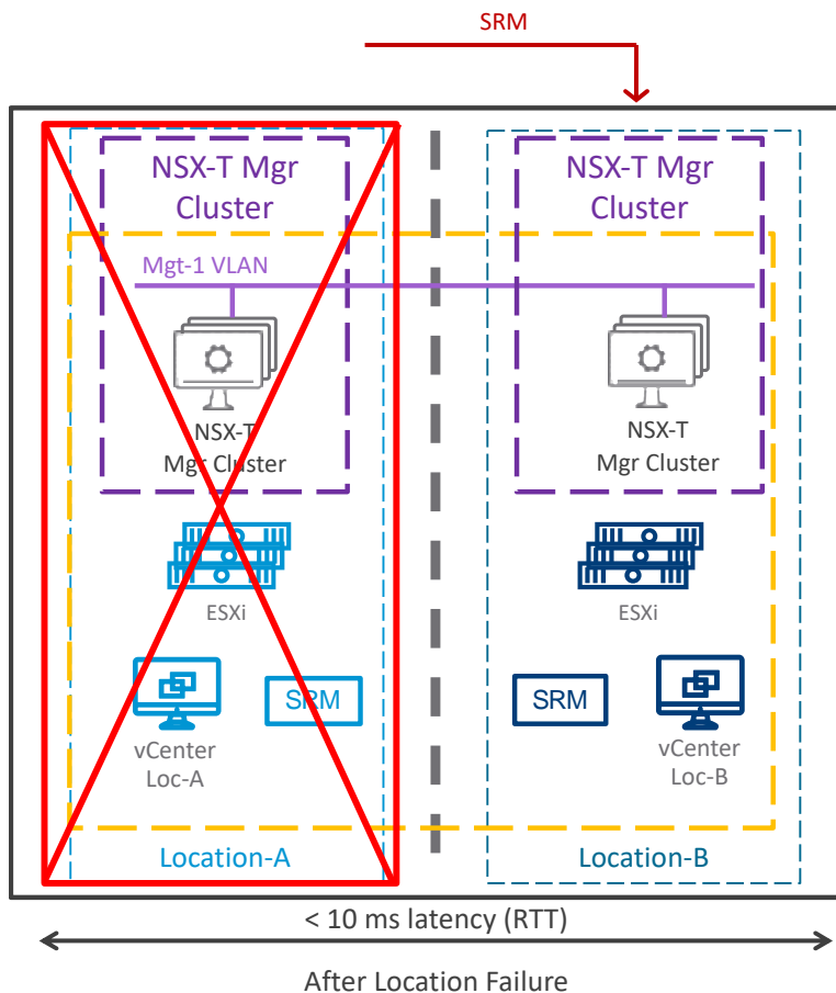
Figure 3-23: Management Plane Deployment Mode 1 Option 1 with SRM – After location failure
