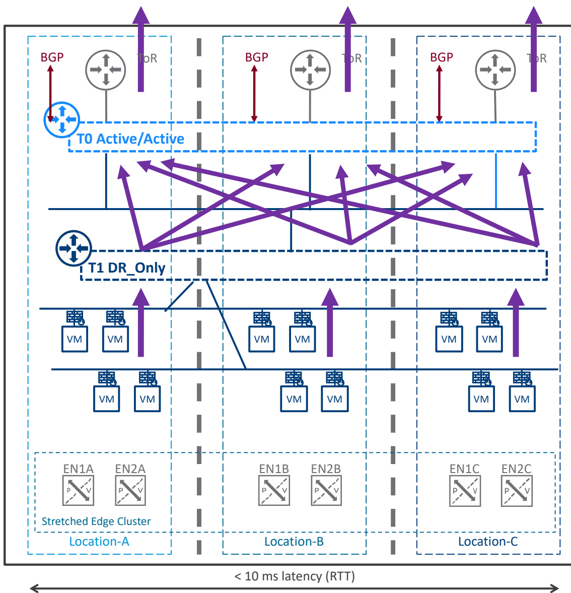
Figure 3-16: NSX-T Multisite Edges - Edge Node Deployment Mode3 with Tier1 DR_Only
