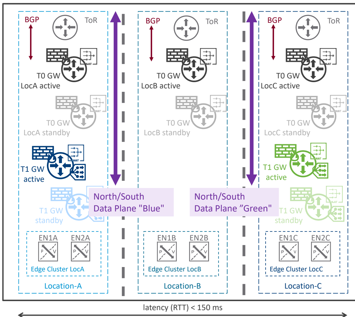
Figure 3-15: NSX-T Multisite Edges - Edge Node Deployment Mode2
