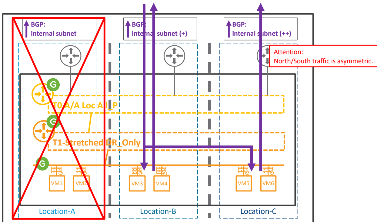
T0 A/A Loc All_P + T1 with No Service – Loss of Location best BGP advertisement
