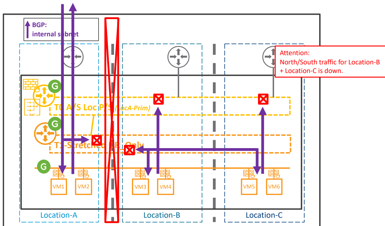
T0 A/S Loc P/S + T1 with No Service – Loss of cross-location communication
