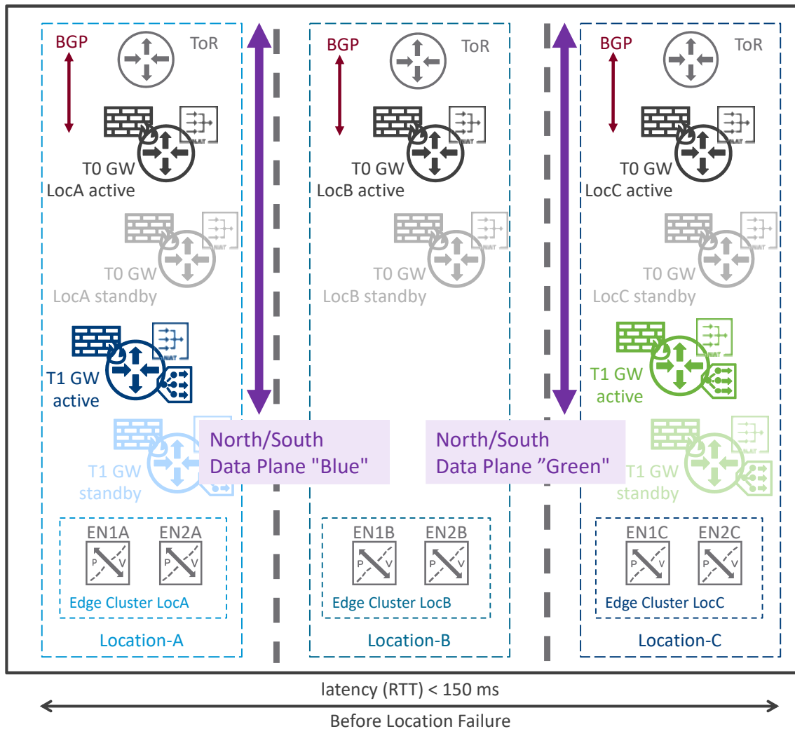
Figure 3-35: Data Plane Deployment Mode2 – Before location failure
