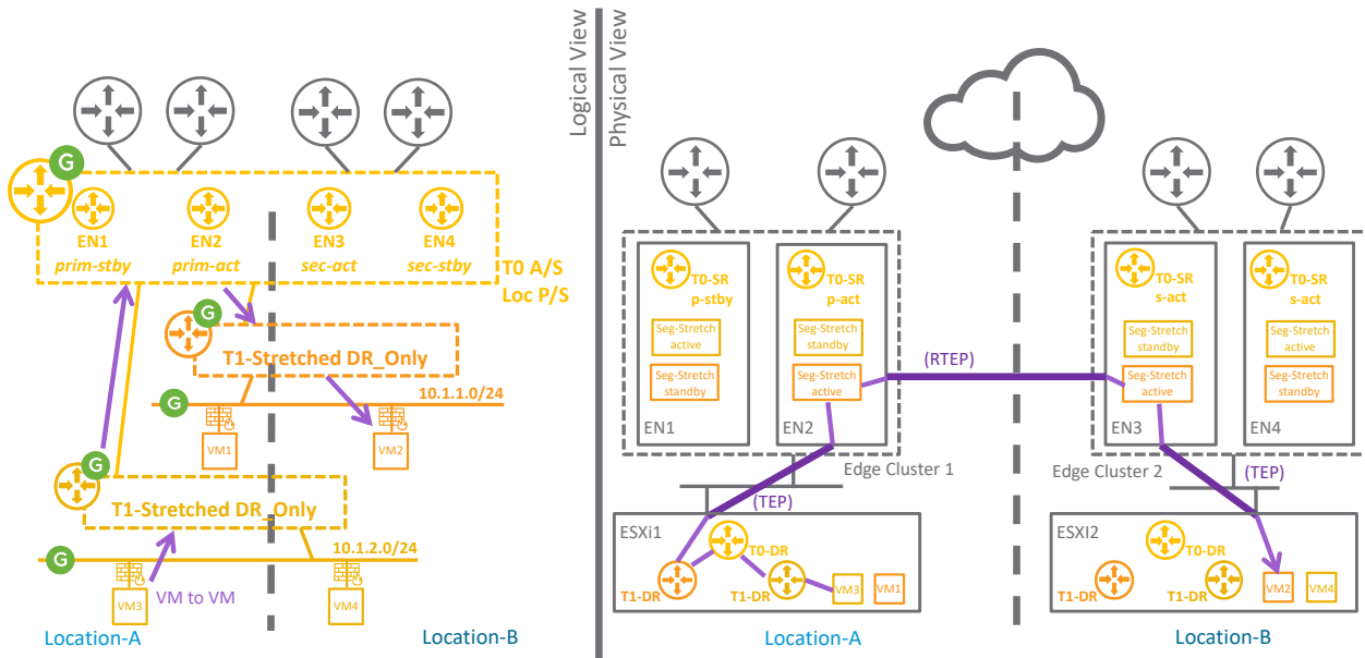
Figure 4-53: NSX-T Federation T1 with SR packet walk2
