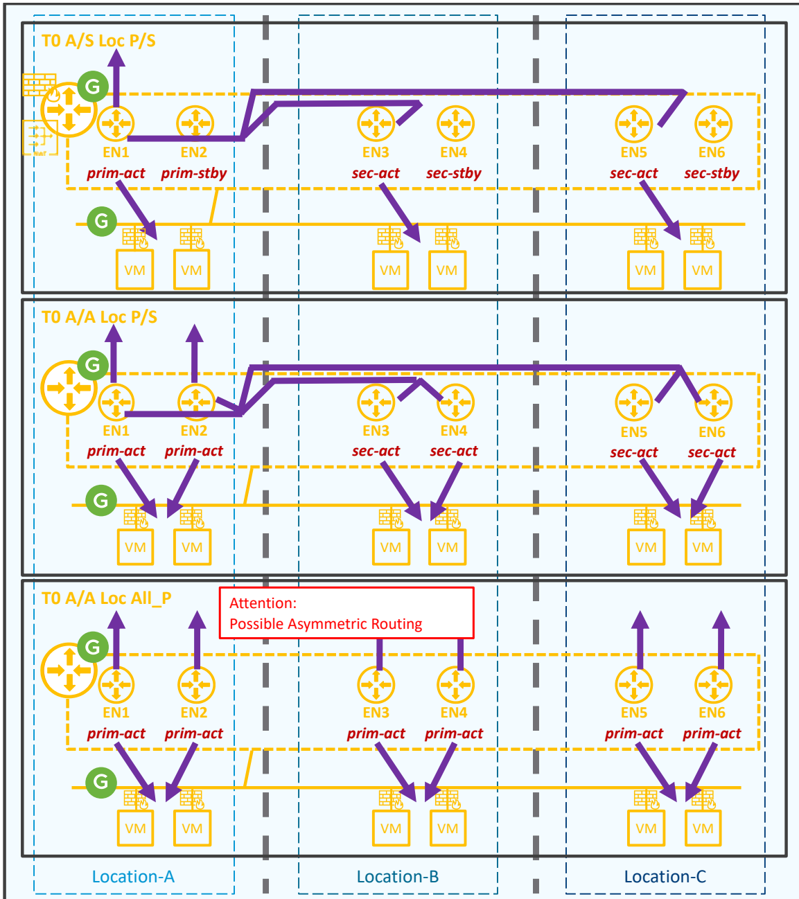
Figure 4-84: NSX-T Federation T0 topologies
