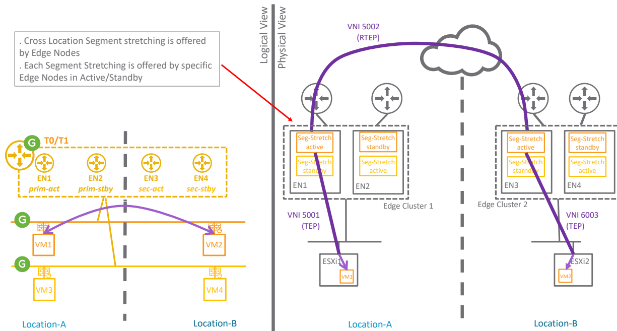
Figure 4-31: NSX-T Federation cross-location logical and physical packet walk
