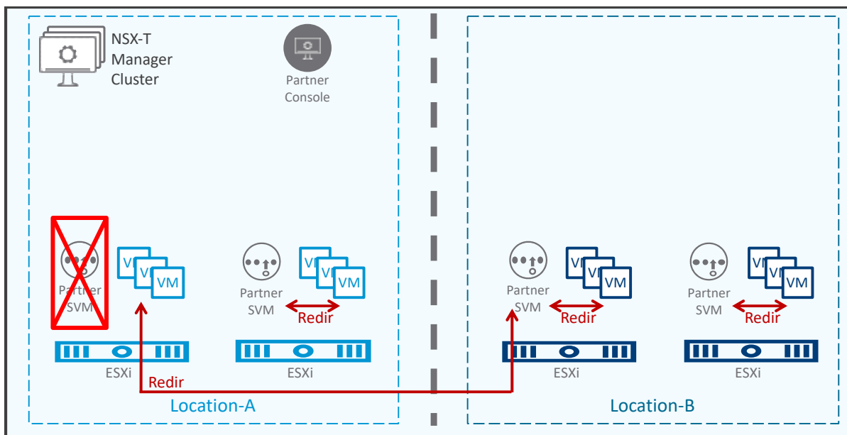
Figure 3-9: NSX-T Multisite Network Introspection and Endpoint Protection redirection – After Partner SVM failure
