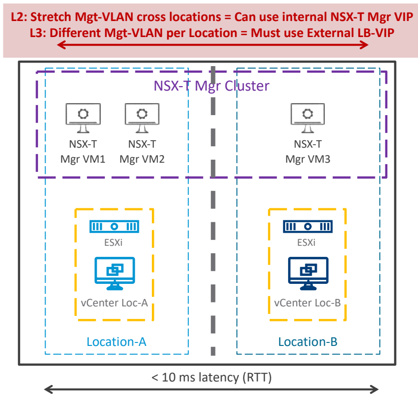
Figure 3-10: NSX-T Multisite Manager Cluster– Management Deployment Mode1 Option1
