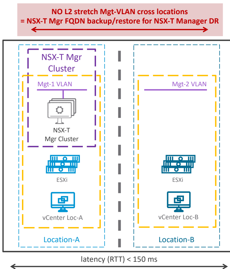
Figure 3-13: NSX-T Multisite Manager Cluster– Management Deployment Mode2 Option2
