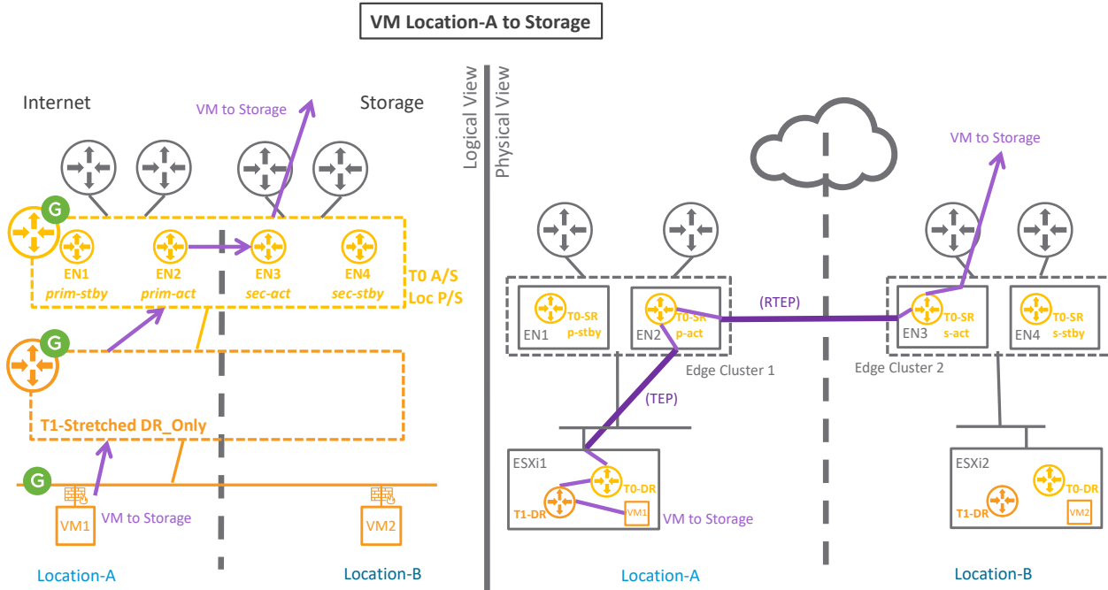
Figure 4-39: NSX-T Federation T0 A/S LocP_S packet walk3
