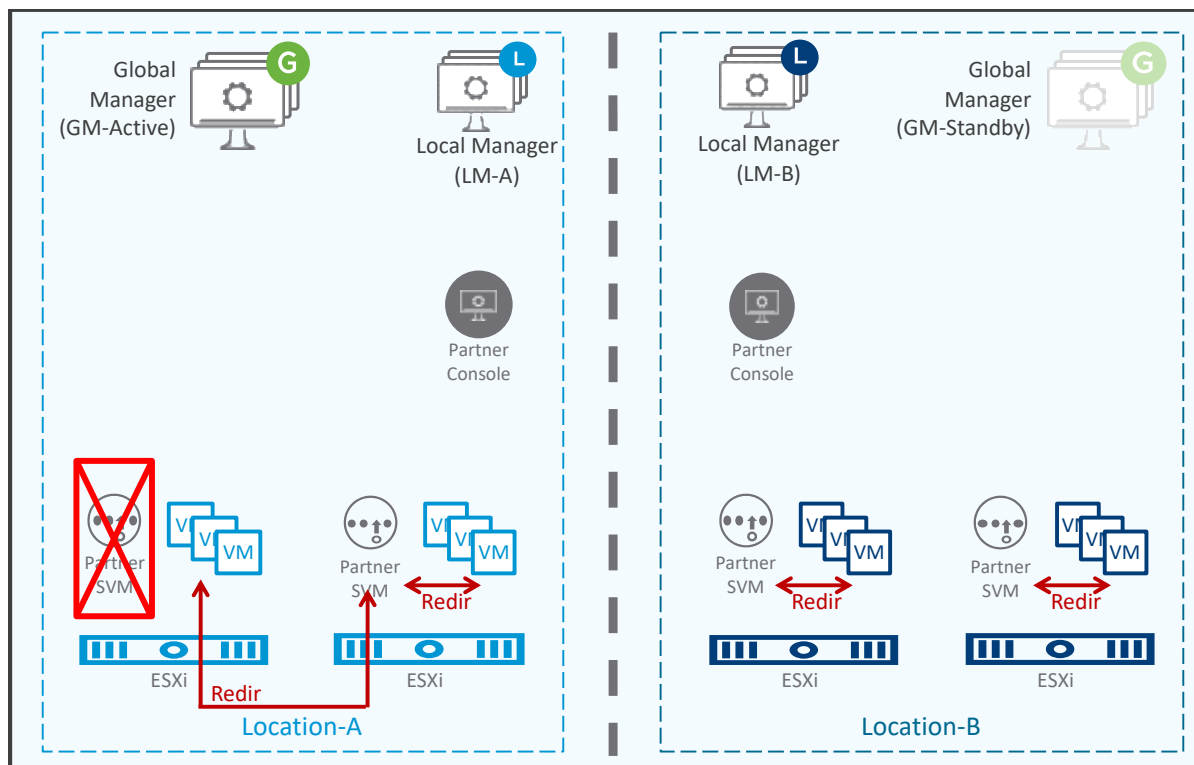
Figure 4-21: NSX-T Multisite Network Introspection and Endpoint Protection redirection – After Partner SVM failure
