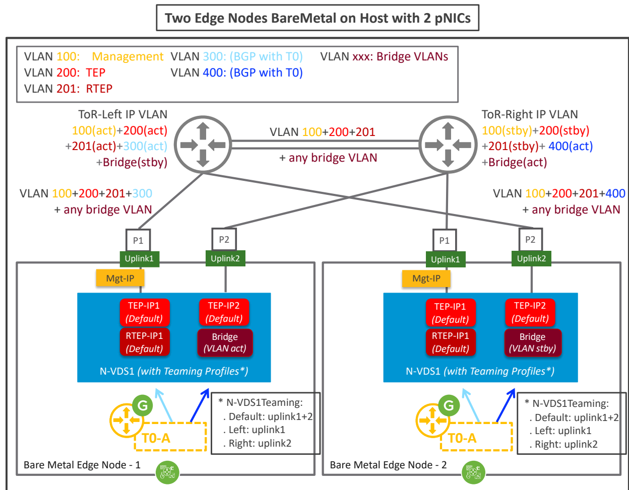
Figure 4-82: NSX-T Federation Edge BareMetal with 2 pNICs recommended configuration
