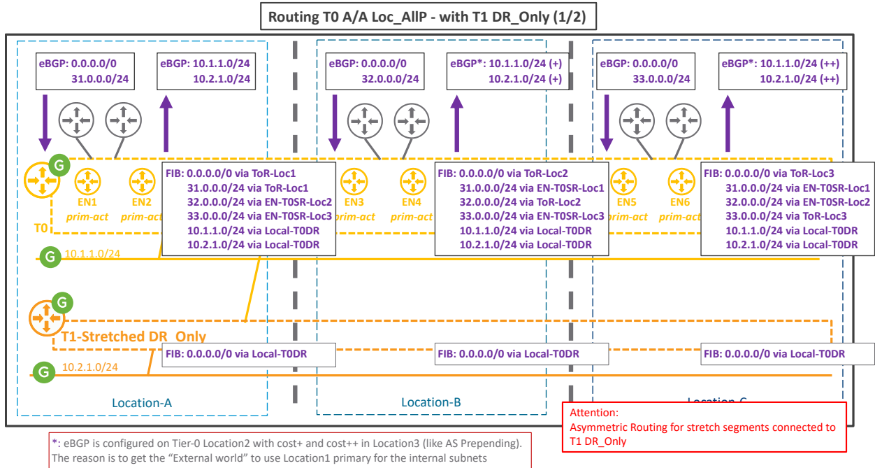
Figure 4-63: T0 Active/Active Location All Primaries with T1_DR_Only
