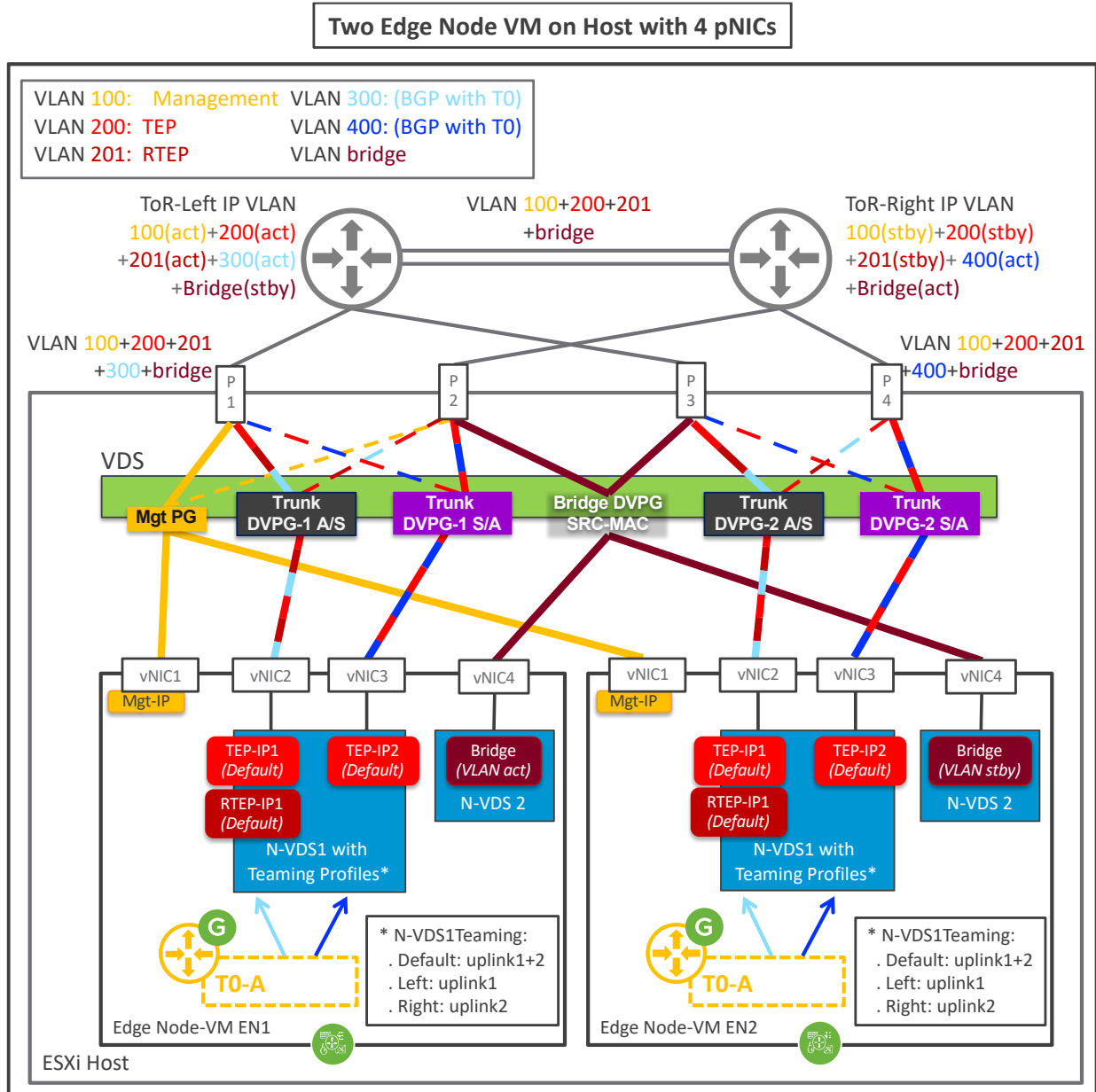
Figure 4-81: NSX-T Federation Edge VM with ESXi 4 pNICs recommended configuration
