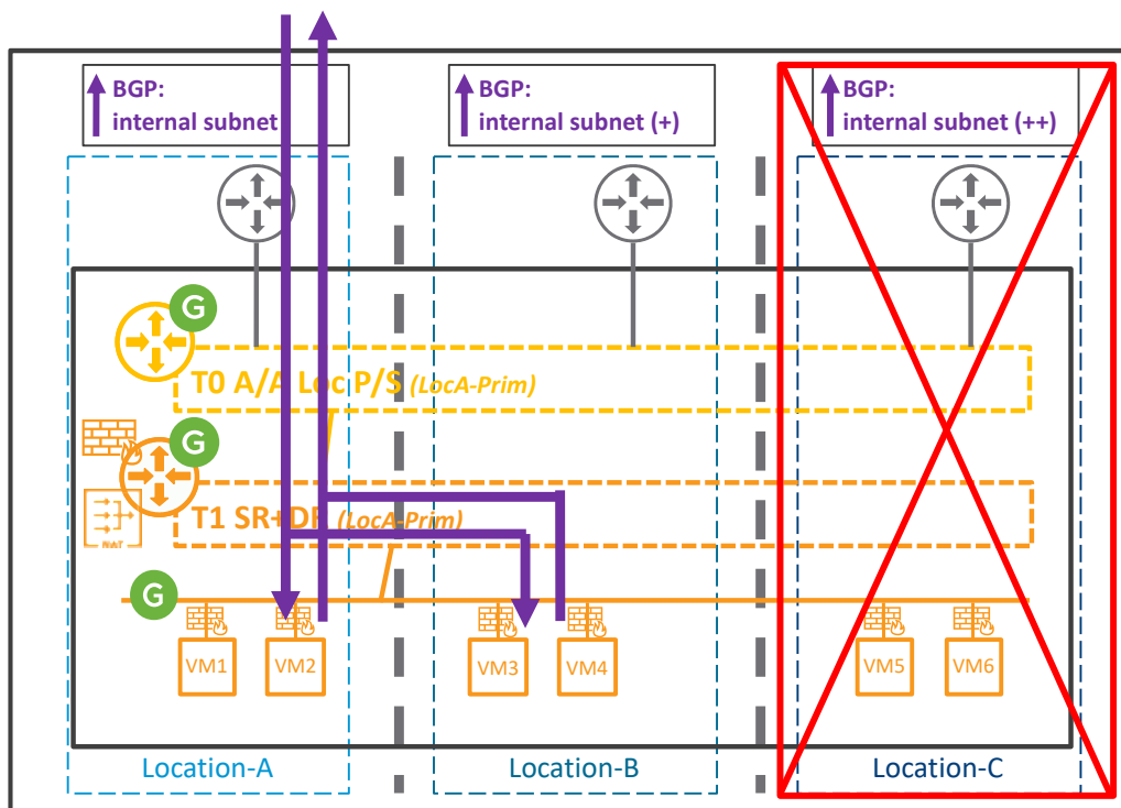
T0 A/A Loc P/S + T1 with Service – Loss of T0/T1 Secondary Location
