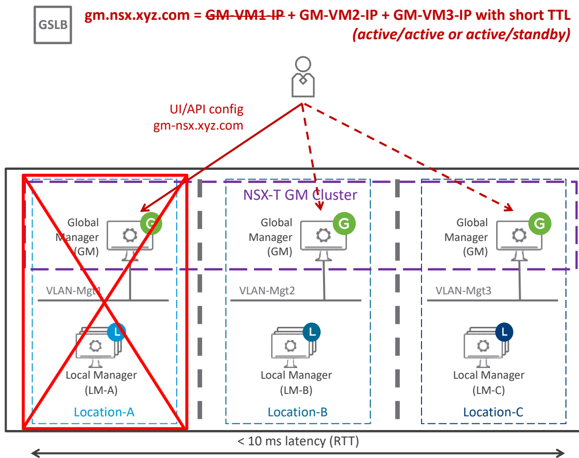
Figure 4-87: NSX-T Federation Management Plane – Use-case metropolitan region with stretched Management VLAN
