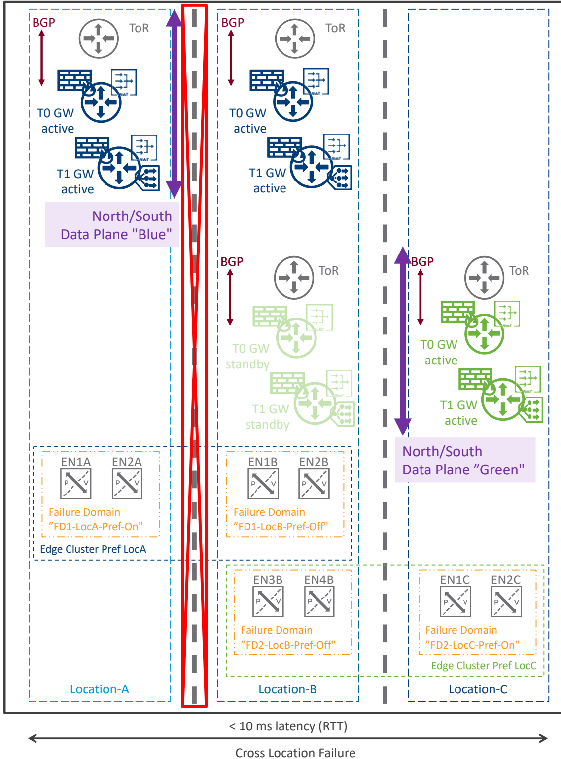
Figure 3-34: Data Plane Deployment Model 1 – After cross-location failure
