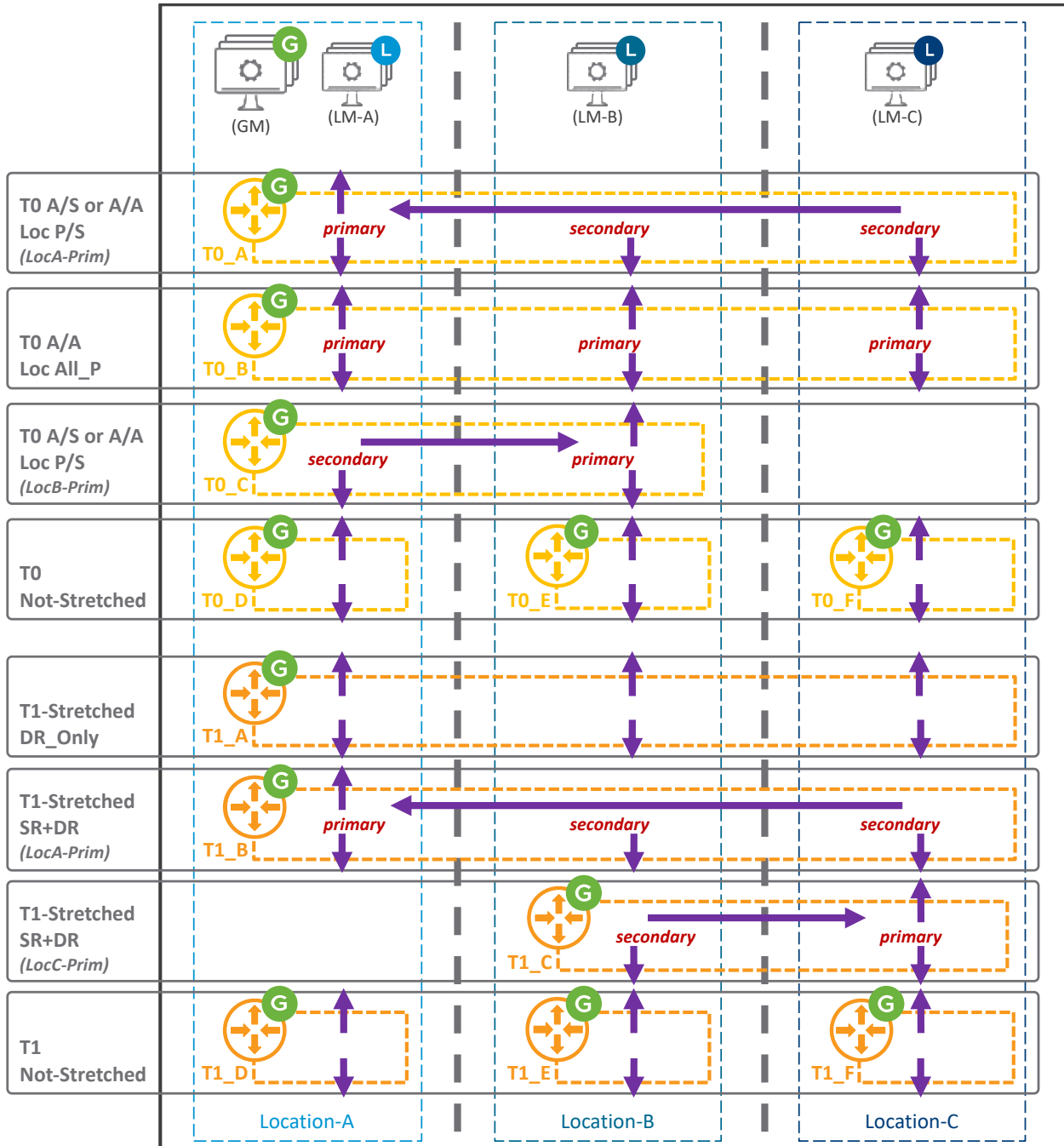
Figure 4-94: Different Tier0/Tier-1 topologies
