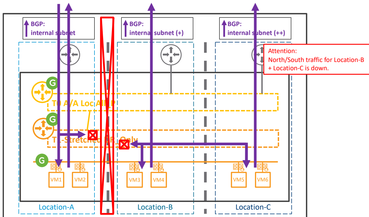
T0 A/A Loc All_P + T1 with No Service – Loss of cross-location communication
