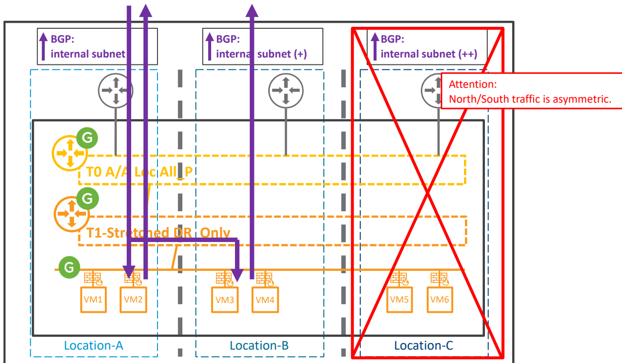
T0 A/A Loc All_P + T1 with No Service – Loss of Location not best BGP advertisement
