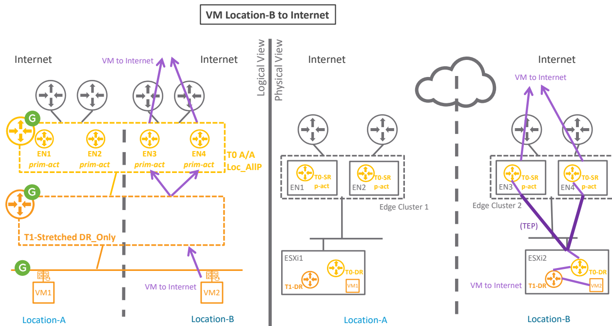
Figure 4-46: NSX-T Federation T0 A/A Loc_AllP packet walk2
