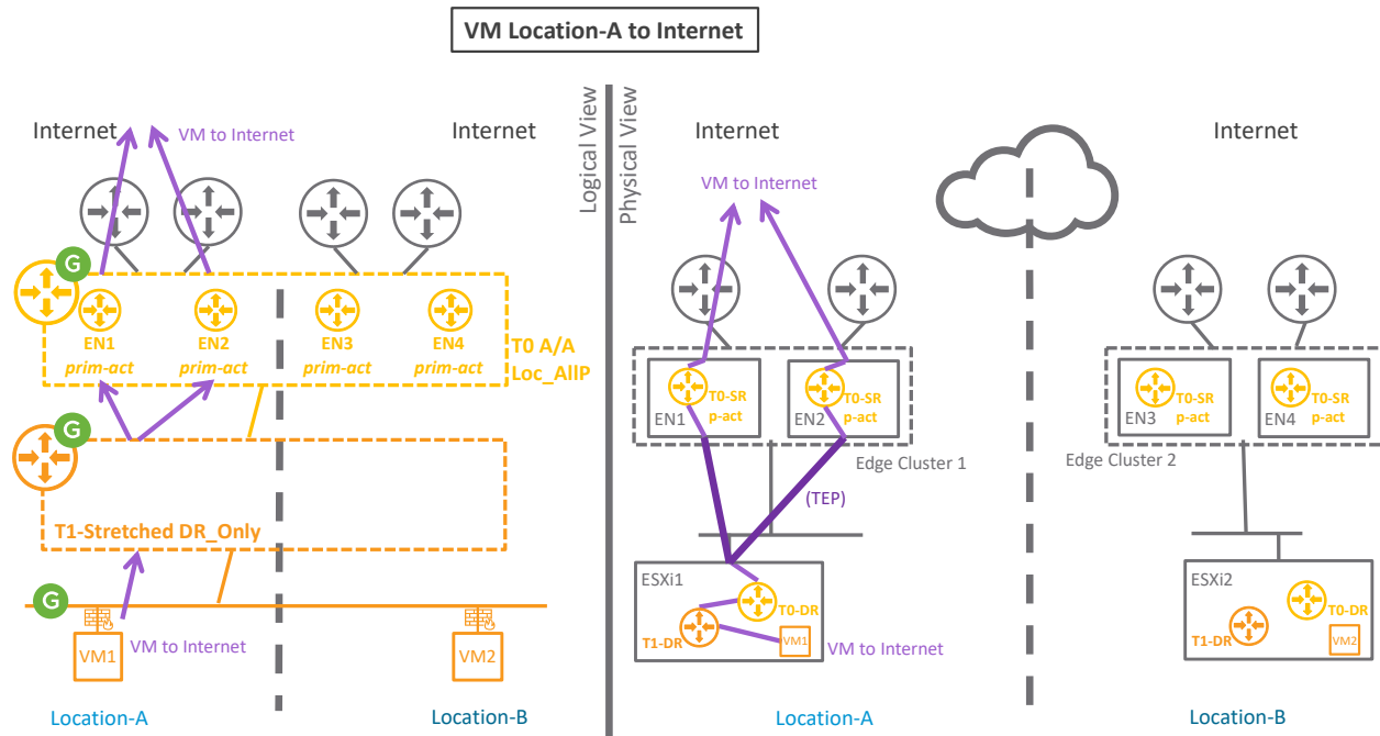
Figure 4-45: NSX-T Federation T0 A/A Loc_AllP packet walk1
