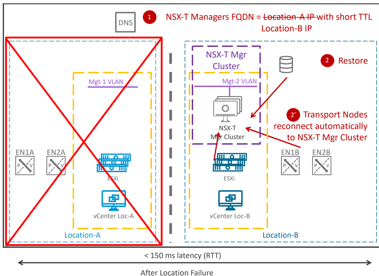
Figure 3-31: Management Plane Deployment Mode2 Option2 – After location failure
