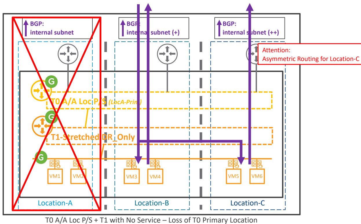
Figure 4-97: T0 A/A Loc P/S with T1-Stretched DR_Only – Loss of T0 Primary Location
