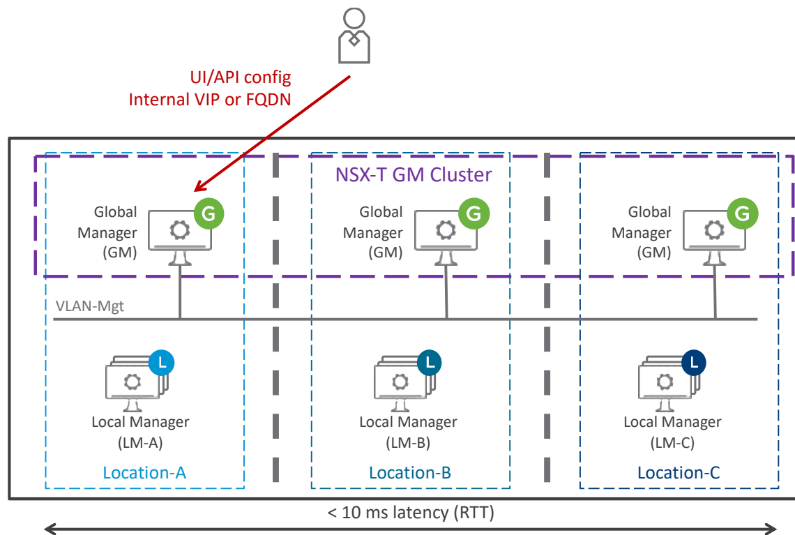
Figure 4-76: NSX-T Federation Management Plane – Use-case metropolitan region with stretched Management VLAN
