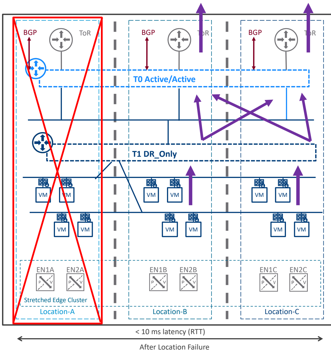
Figure 3-40: Data Plane Deployment Mode3 with Tier1 DR_Only – After location failure
