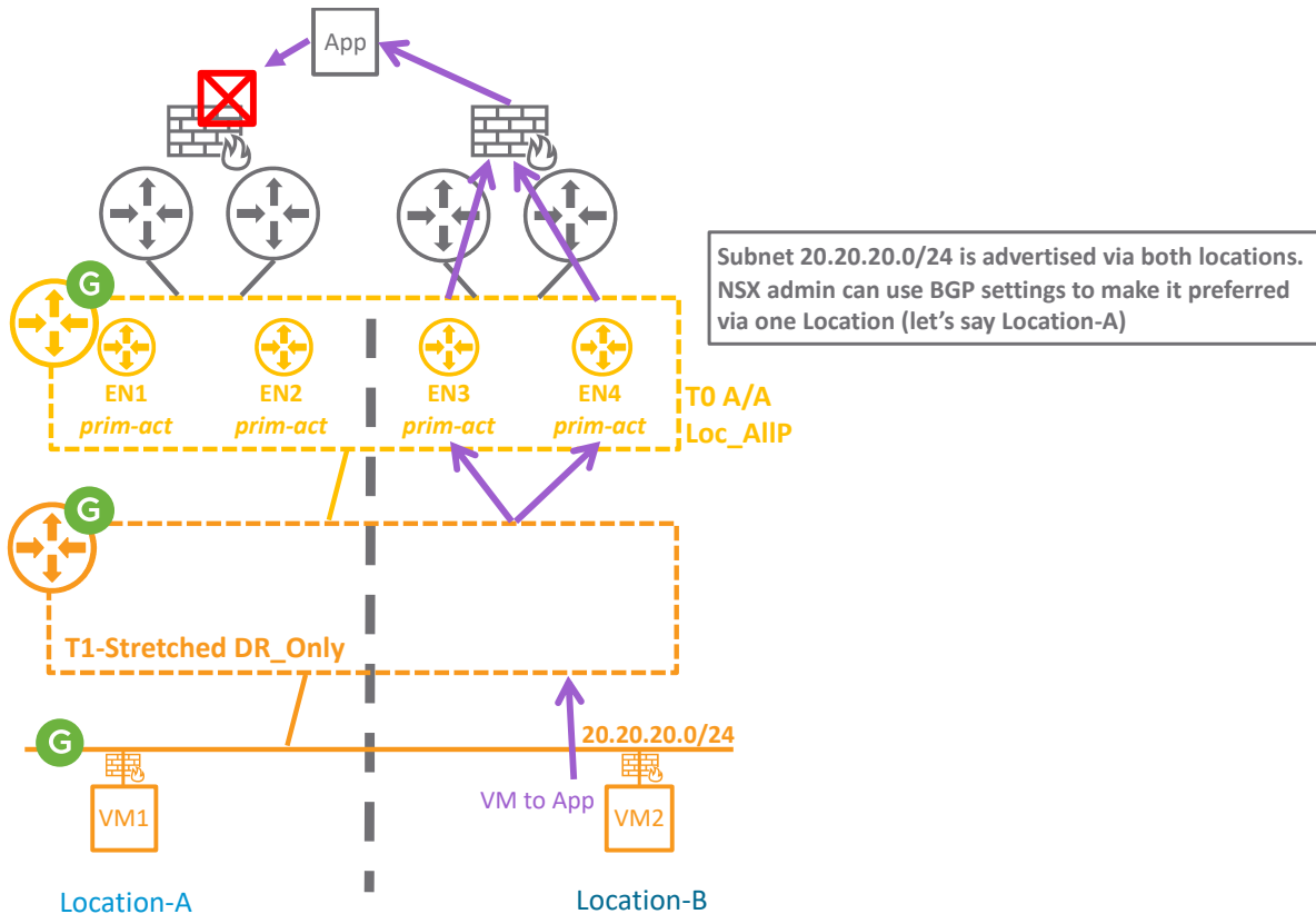
Figure 4-85: NSX-T Federation TO A/A Loc_AllP asymmetric routing
