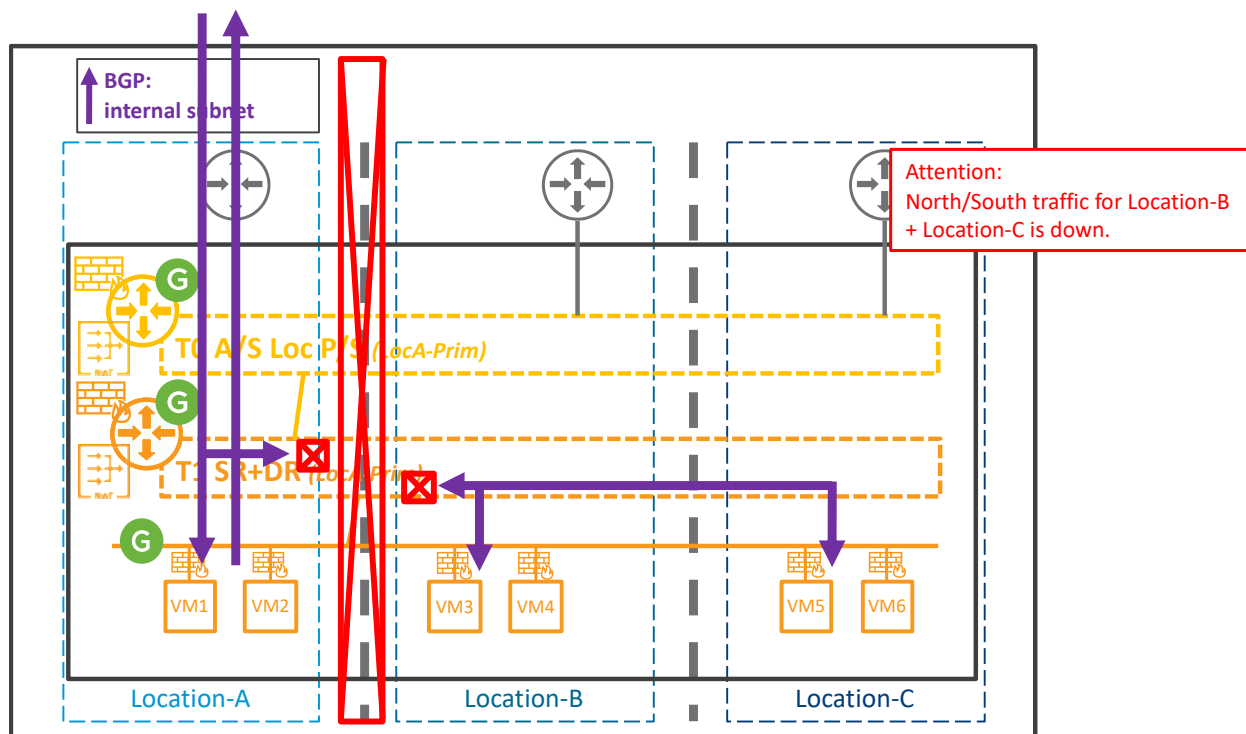
T0 A/S Loc P/S + T1 with Service – Loss of cross-location communication
