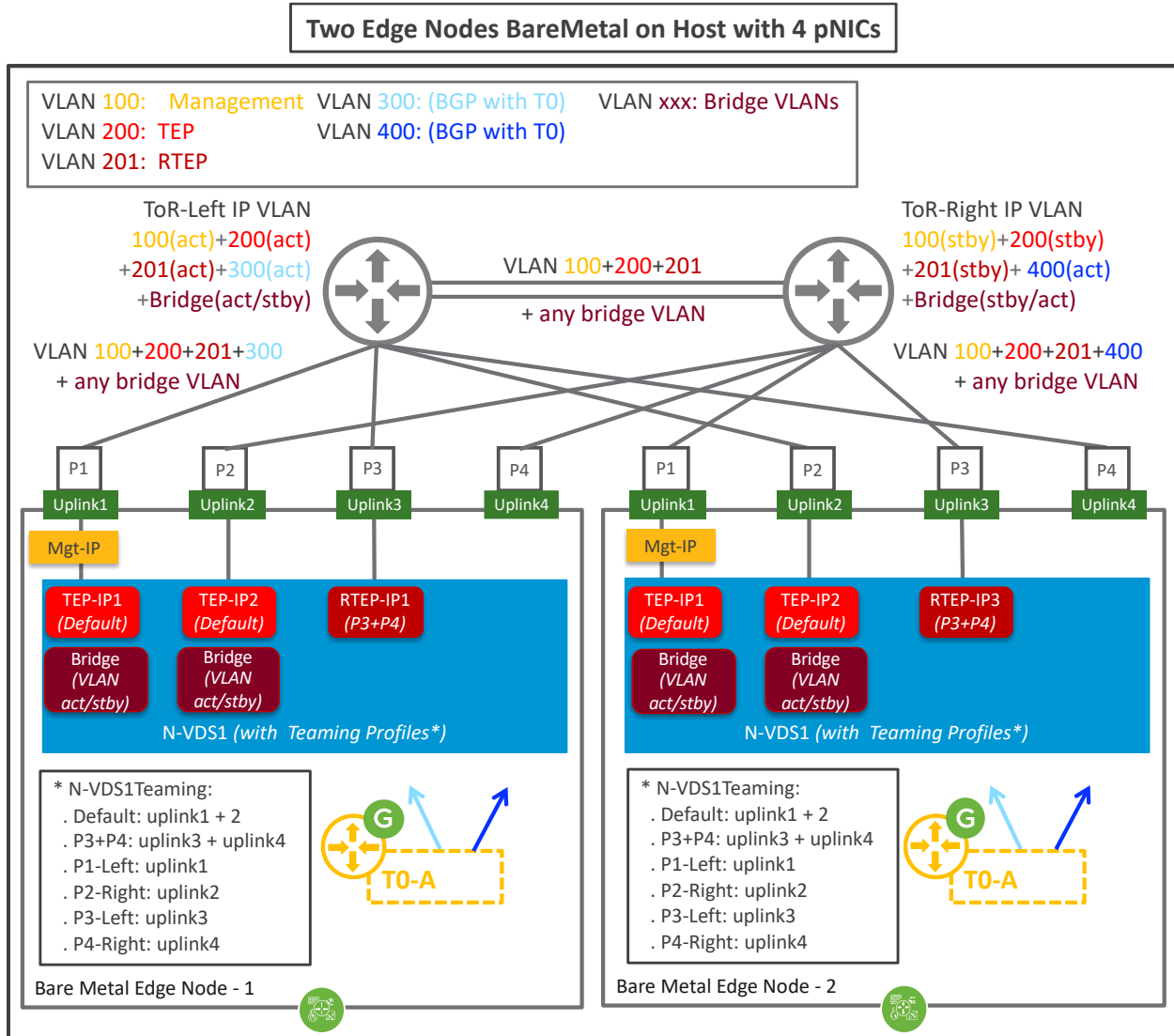
Figure 4-83: NSX-T Federation Edge BareMetal with 4 pNICs recommended configuration
