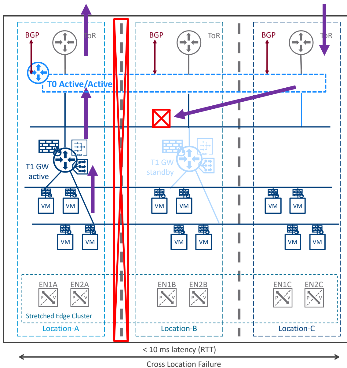
Figure 3-43: Data Plane Deployment Mode3 with Tier1 with Services – After cross-location failure
