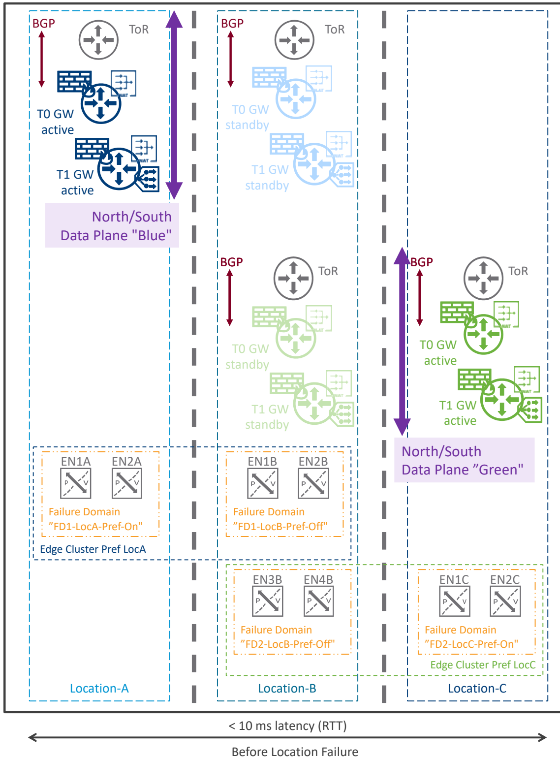
Figure 3-32: Data Plane Deployment Model 1 – Before location failure
