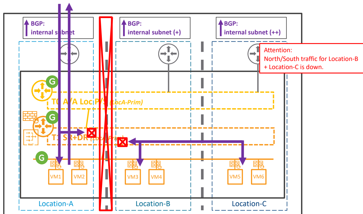
T0 A/A Loc P/S + T1 with Service – Loss of cross-location communication
