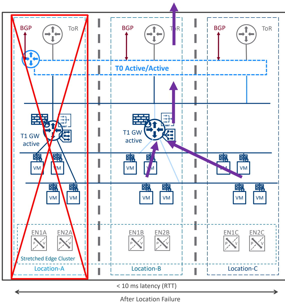
Figure 3-41: Data Plane Deployment Mode3 with Tier1 with Services – After location failure
