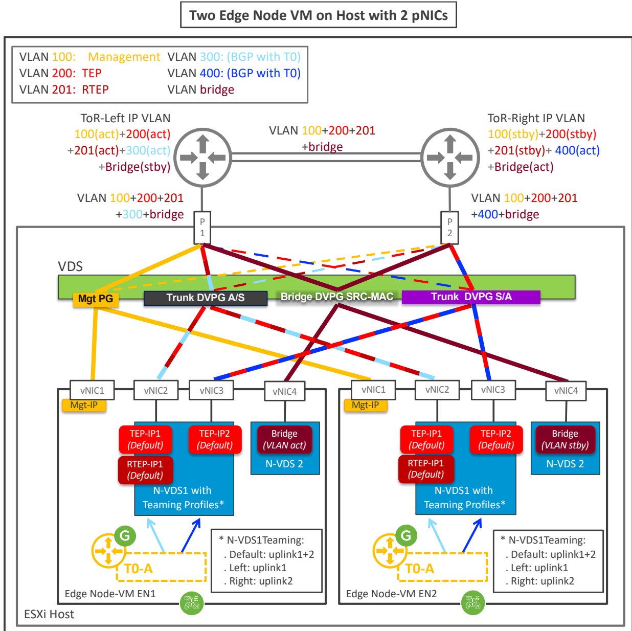
Figure 4-80: NSX-T Federation Edge VM with ESXi 2 pNICs recommended configuration
