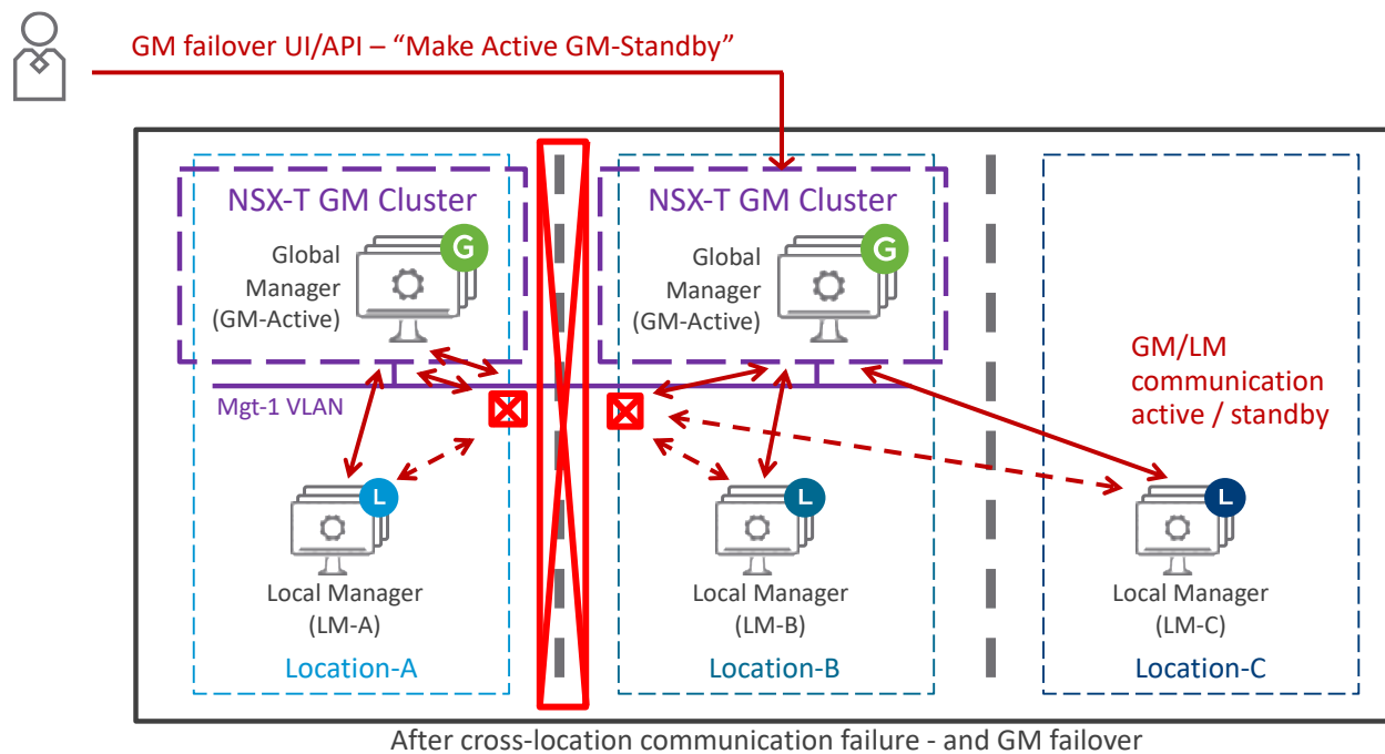
Figure 4-91: NSX-T Federation GM service after cross-location failure hosting the GM-Active service+ GM failover
