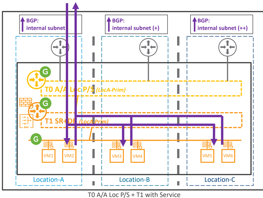
Figure 4-111: T0 A/A Loc P/S with T1 A/S Loc P/S
