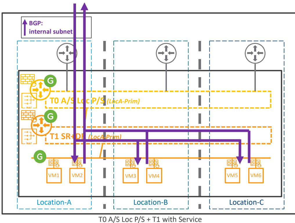
Figure 4-107: T0 A/S Loc P/S with T1 A/S Loc P/S
