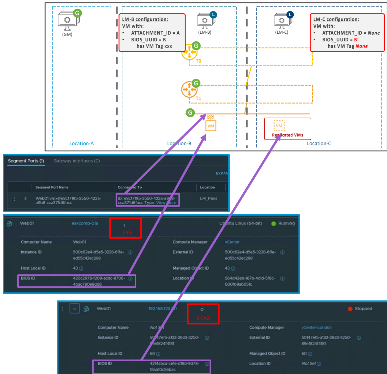
Figure 4-123: VM inventory information in different LMs prior to SRM recovery without GM Sync VM Tag configuration
