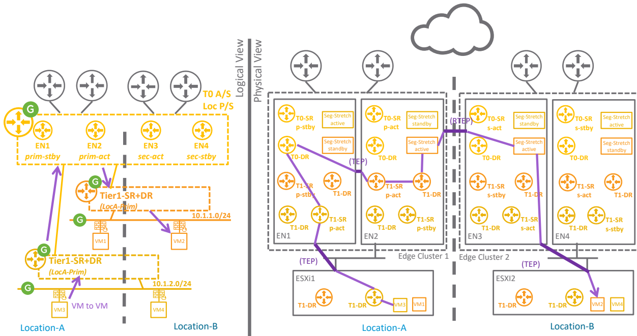
Figure 4-54: NSX-T Federation T1 with SR packet walk3
