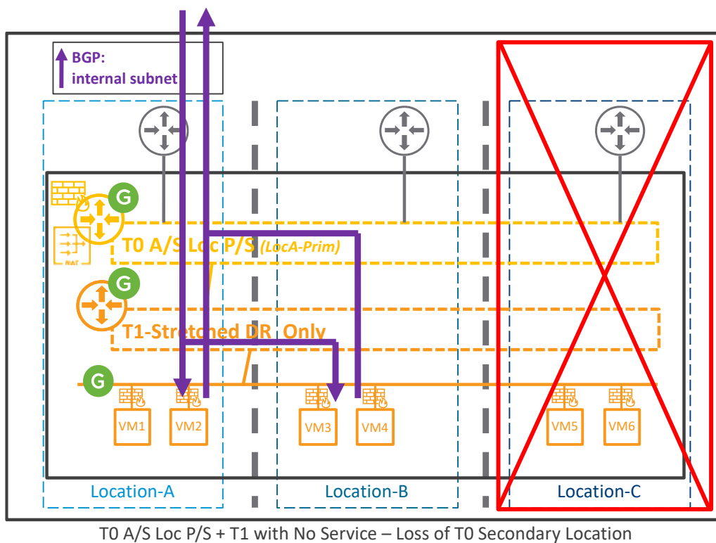
Figure 4-104: T0 A/S Loc P/S with T1-Stretched DR_Only – Loss of T0 Secondary Location
