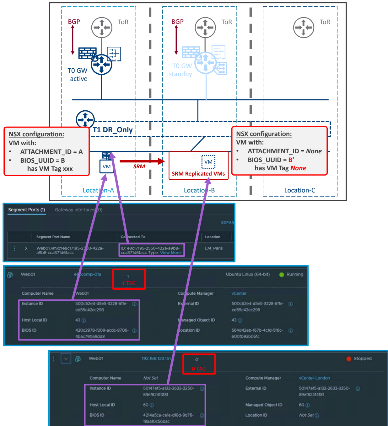
Figure 3-44: Compute VMs before location failure
