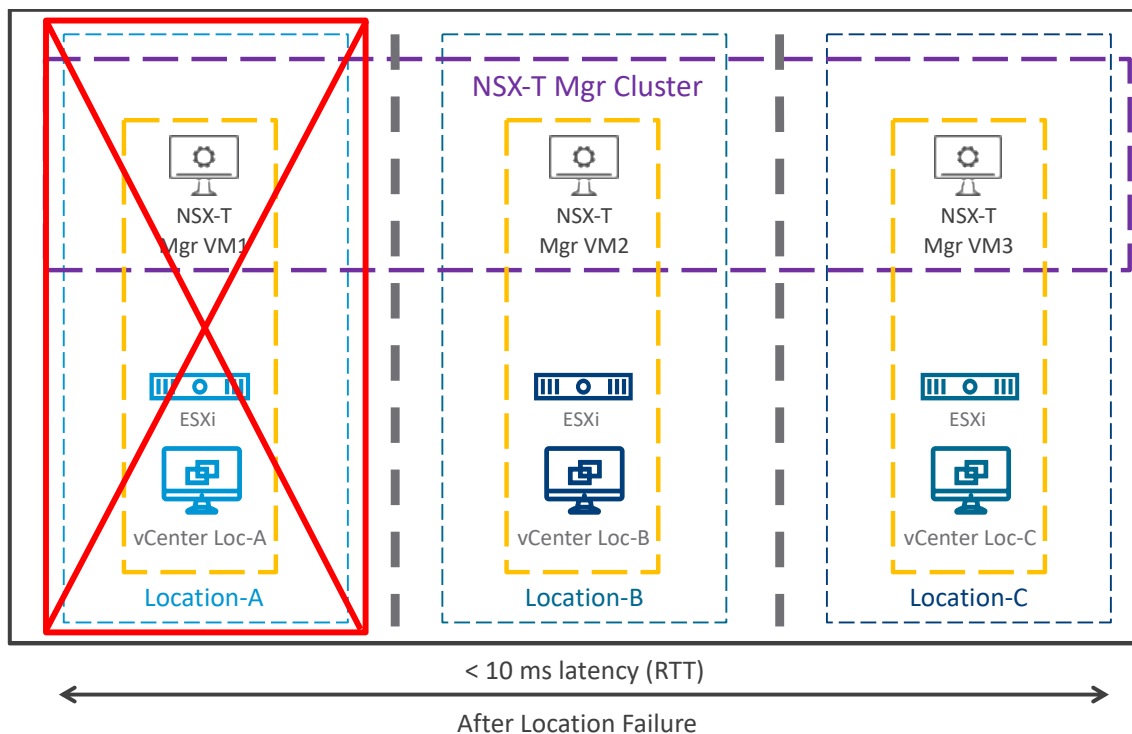
Figure 3-27: Management Plane Deployment Mode1 Option3 – After location failure
