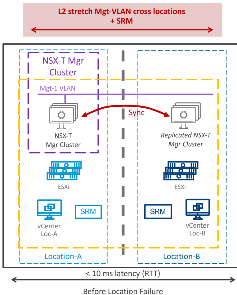
Figure 3-22: Management Plane Deployment Model Option 1 with SRM – Before location failure
