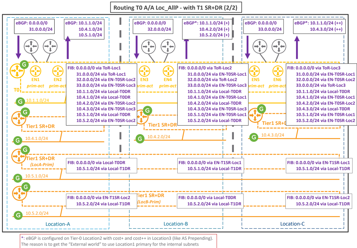
Figure 4-64: T0 Active/Active Location All Primaries with T1_SR+DR
