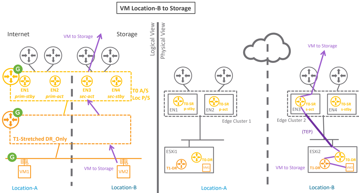
Figure 4-40: NSX-T Federation T0 A/S LocP_S packet walk4
