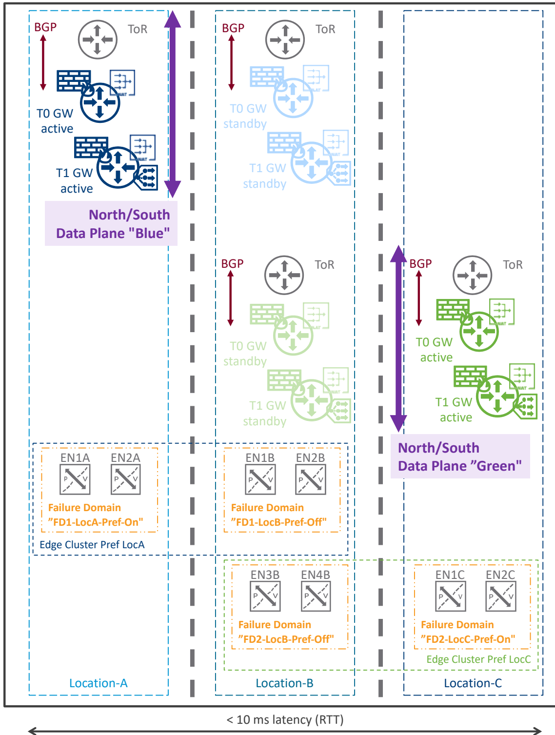
Figure 3-14: NSX-T Multisite Edges - Edge Node Deployment Model 1
