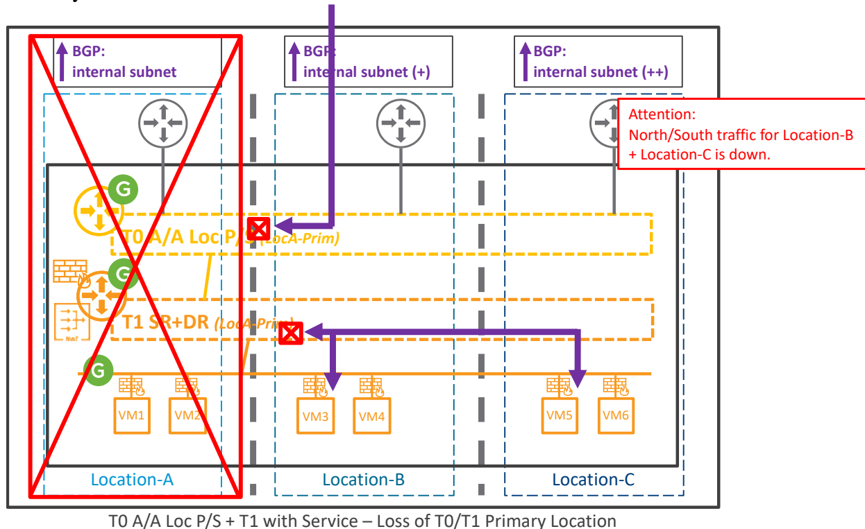
Figure 4-113: T0 A/A Loc P/S with T1 A/S Loc P/S – Loss of T0/T1 Primary Location
