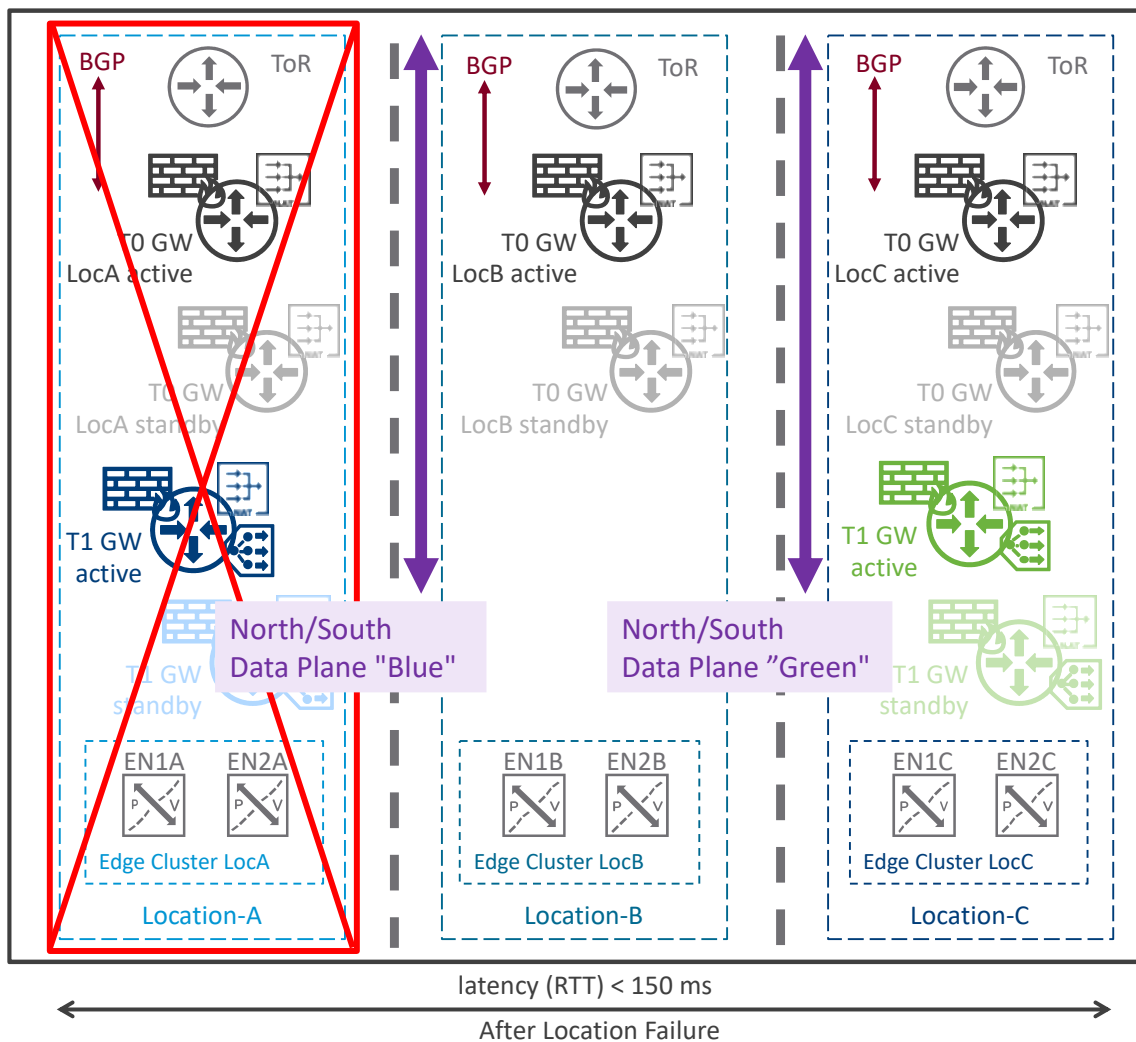
Figure 3-36: Data Plane Deployment Mode2 – After location failure
